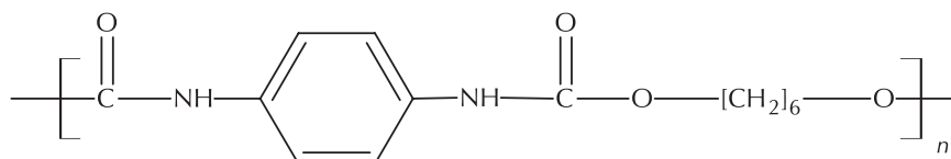
poli[(1,4-diizocijanatobenzen)-alt-(heksan-1,6-diol)]
