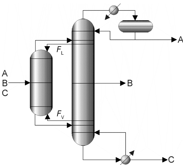
Fig. 1 – Structure of the Petlyuk column
